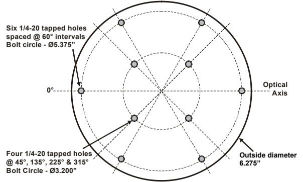
1100GTO Dec. Top Plate Mounting Hole Pattern
