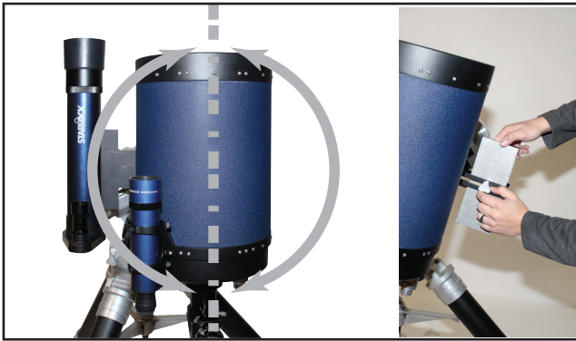
Fig 31: Balancing the StarLock assembly
