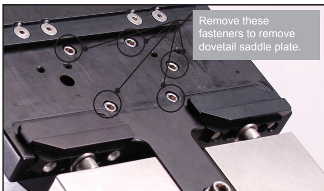
Fig 15: Access to left saddle fastener revealed.
