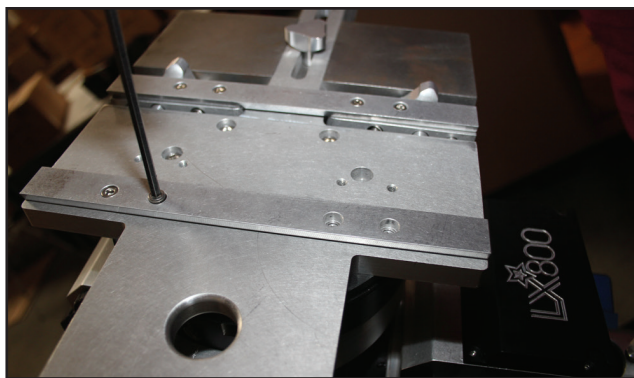
Fig 22: Replace the saddle plate
