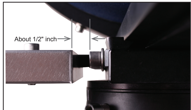
Fig 46: Gap of 1/2" between cap screw and weight.
