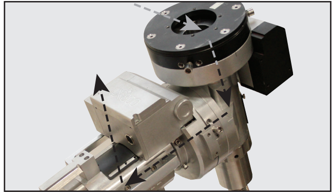
Fig 19: Route of cable from StarLock module
