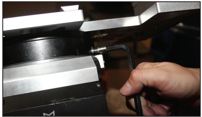
Fig 11: Tighten Clutch.
