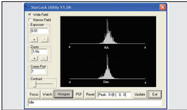
Fig 42: Typical Histogram
