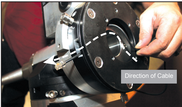
Fig 17: Routing cable under the saddle plate.
