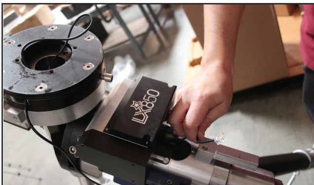
Fig 18: Pulling cable out to connect to control panel.
