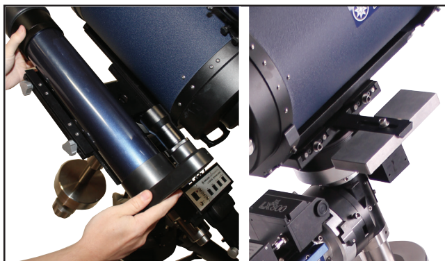
Fig 26: Mounting StarLock to the saddle plate. Attach StarLock counterweight.
