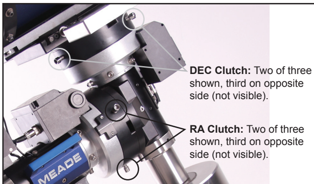
Fig 10: DEC and RA Clutch Locations
